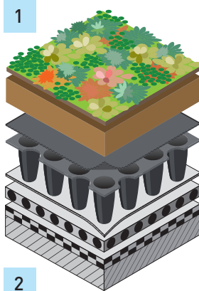
ND 5+1 Drainagesystem
